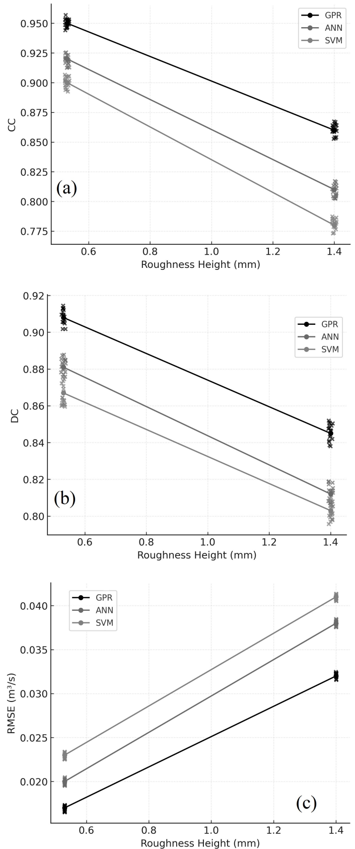
Fig. 8 Variation of machine-learning models under different bed roughness heights: (a) CC, (b) DC, and (c) RMSE
